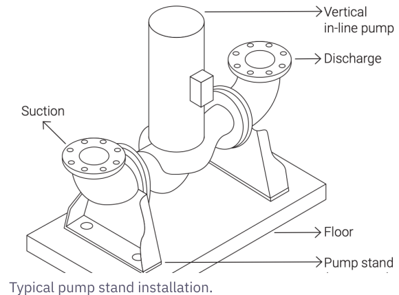
Typical pump stand installation.
