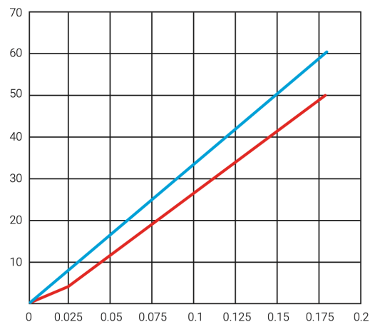
Load (psi) versus deflection (in). Blue: RP-18. Red: DP-18.
