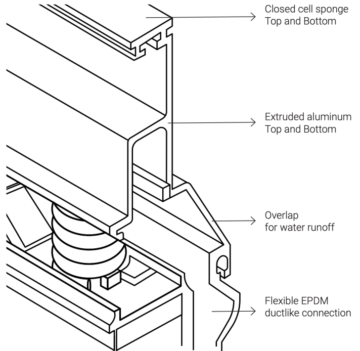
Section view of the rail.
